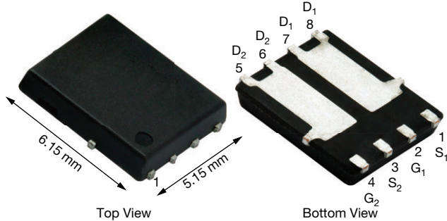
PowerPAK® SO-8 Dual
