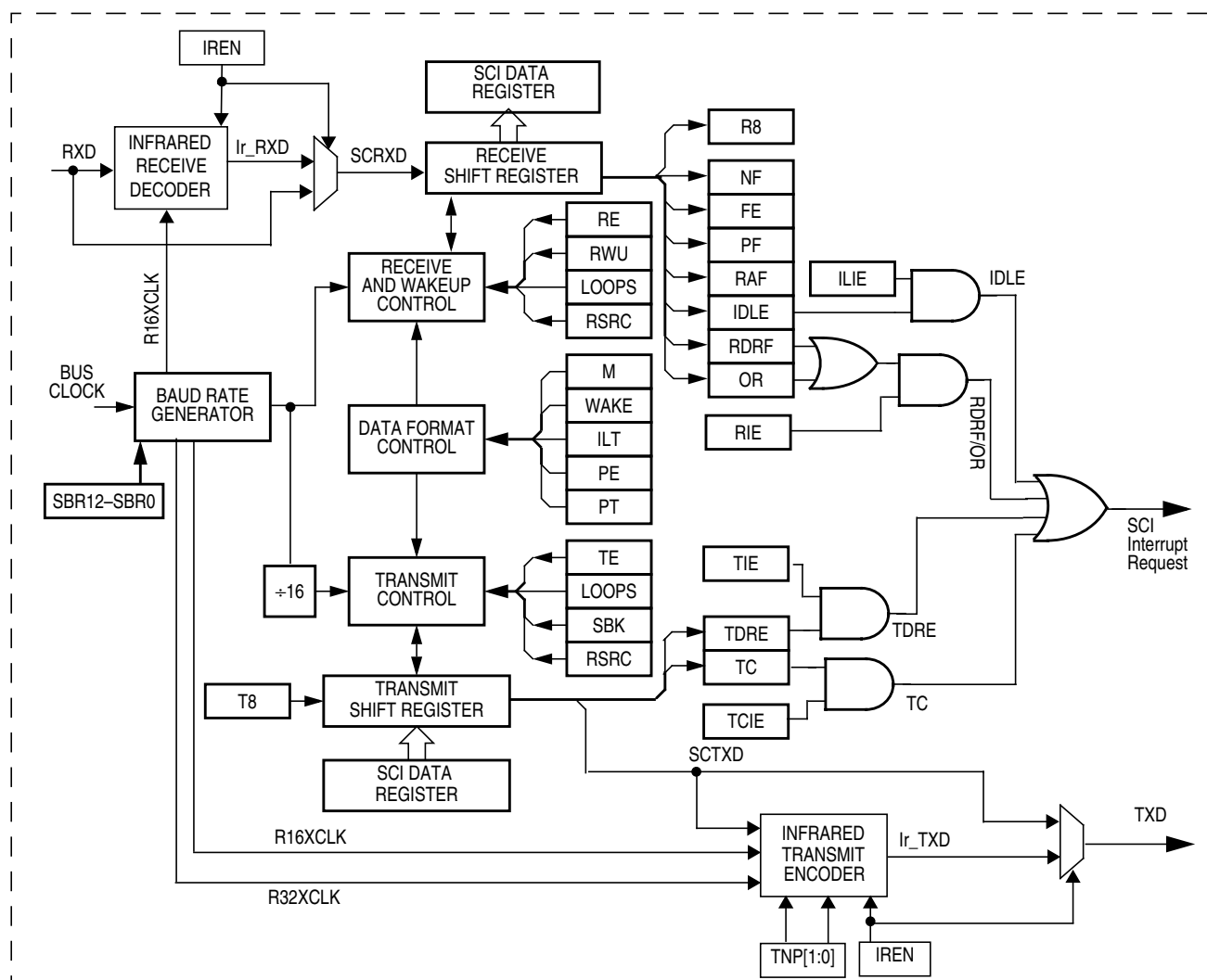
Figure 8-11. Detailed SCI Block Diagram
