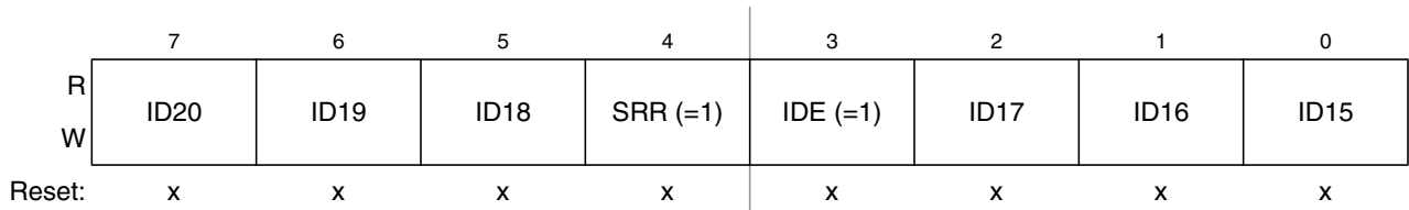
Figure 18-27. Identifier Register 1 (IDR1) — Extended Identifier Mapping
