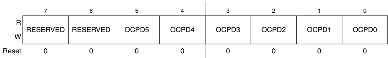
Figure 22-20. Output Compare Pin Disconnect Register (OCPD)
