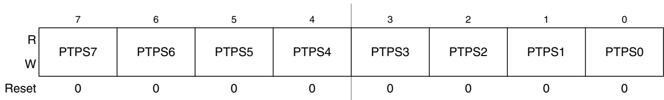
Figure 22-21. Precision Timer Prescaler Select Register (PTPSR)
