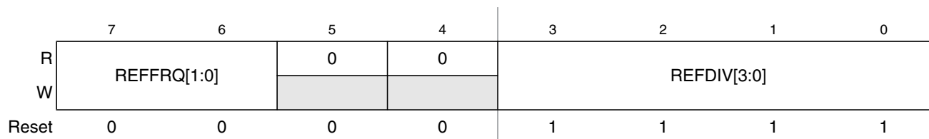
Figure 10-5. S12CPMU Reference Divider Register (CPMUREFDIV)
