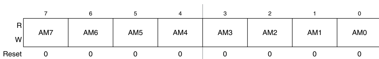
Figure 18-22. MSCAN Identifier Mask Registers (First Bank) — CANIDMR0–CANIDMR3
