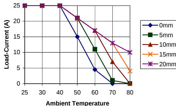
GNR90mm 25A Allowable Load-Current (Horizontal Spacing)
