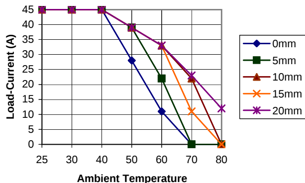
GNR45mm 45A Allowable Load-Current (Horizontal Spacing)
