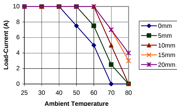
GNR22.5mm 10A Allowable Load-Current (Horizontal Spacing)
