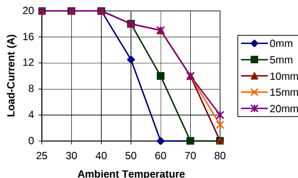
GNR22.5mm 20A Allowable Load-Current (Horizontal Spacing)
