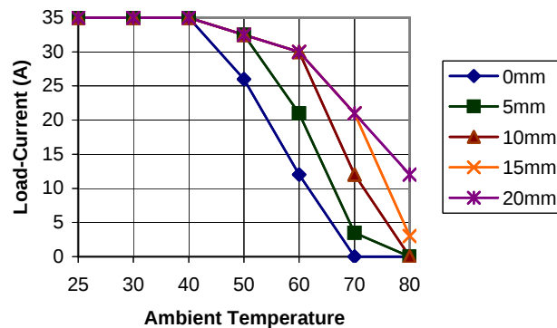
GNR45mm 35A Allowable Load-Current (Horizontal Spacing)
