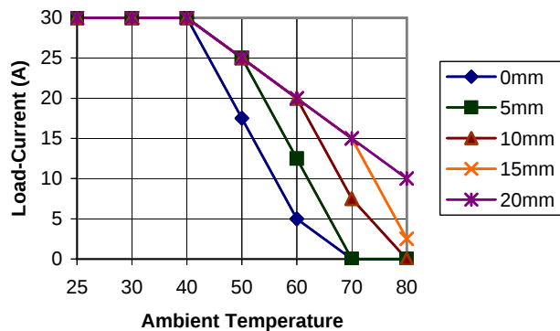
GNR22.5mm 30A Allowable Load-Current (Horizontal Spacing)
