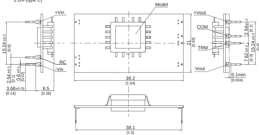
2.DIP(type C)
