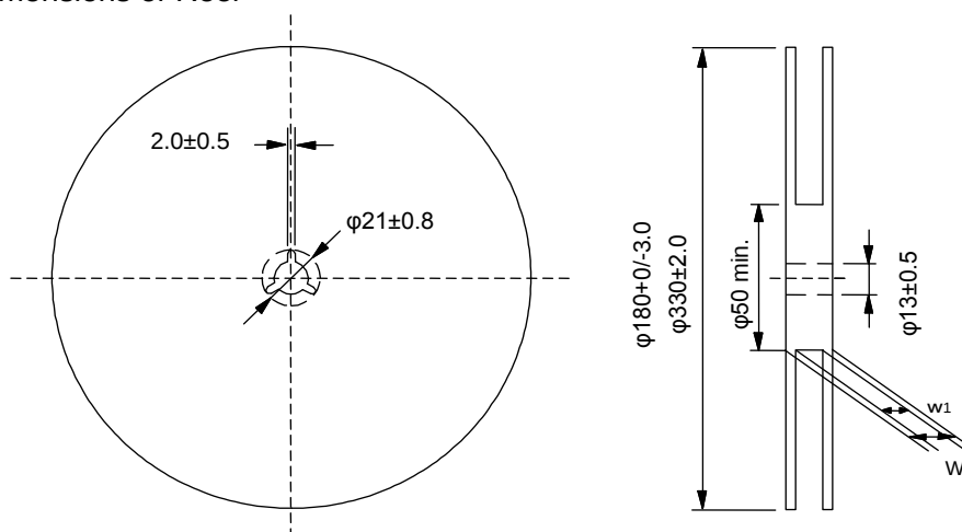
Fig.3 Taping Diagram
