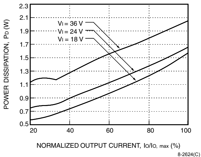
Figure 25. LC005B Power Dissipation vs. Output Current
