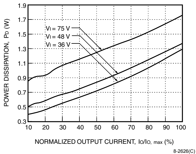
Figure 26. LW005F Power Dissipation vs. Output Current
