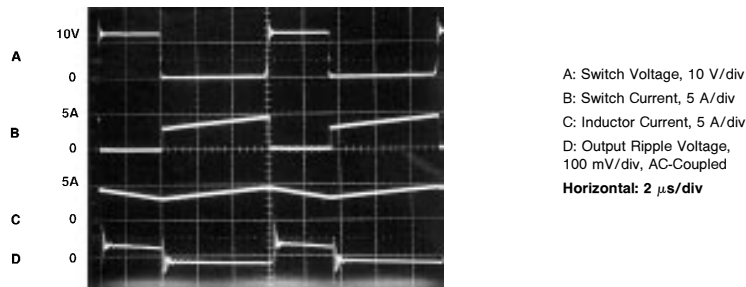
FIGURE 34. Switching Waveforms
