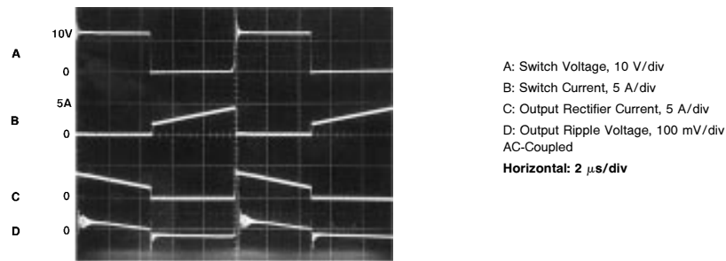
FIGURE 5. Switching Waveforms
