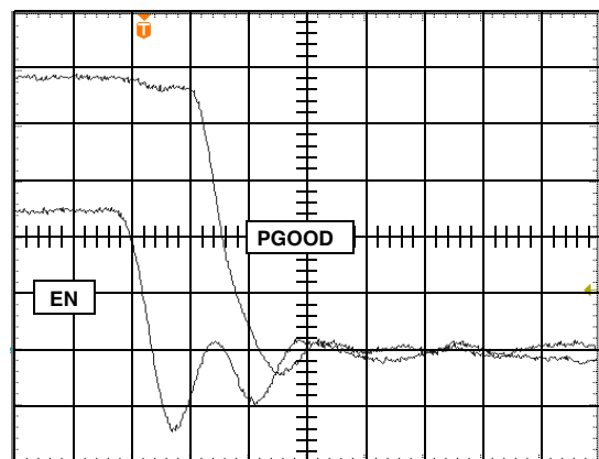
FIGURE 8. EN LOW to PGOOD
