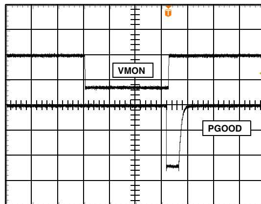
FIGURE 9. VMON LOW to PGOOD
