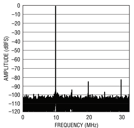
LTC2258-14: 8k Point FFT, f_{IN} = 140\text{MHz} , -1\text{dBFS} , 65Msps
