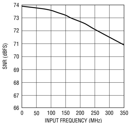
LTC2258-14: SNR vs Input Frequency, -1\text{dB} , 2V Range, 65Msps
