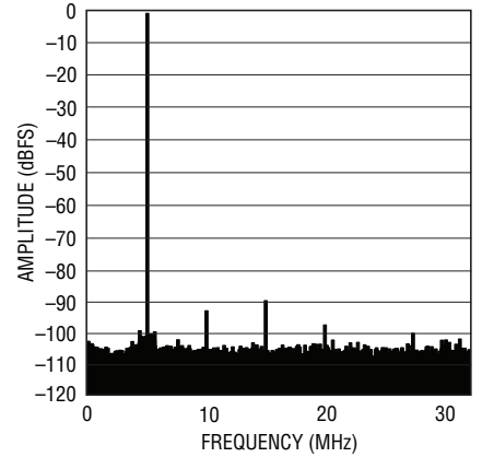
LTC2258-14: 8k Point FFT, f_{IN} = 5\text{MHz} , -1\text{dBFS} , 65Msps
