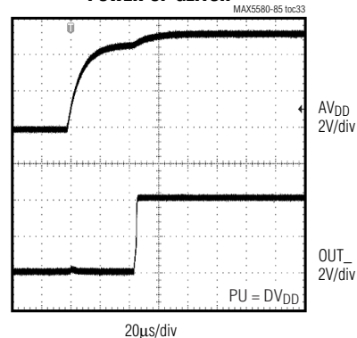
POWER-UP GLITCH
