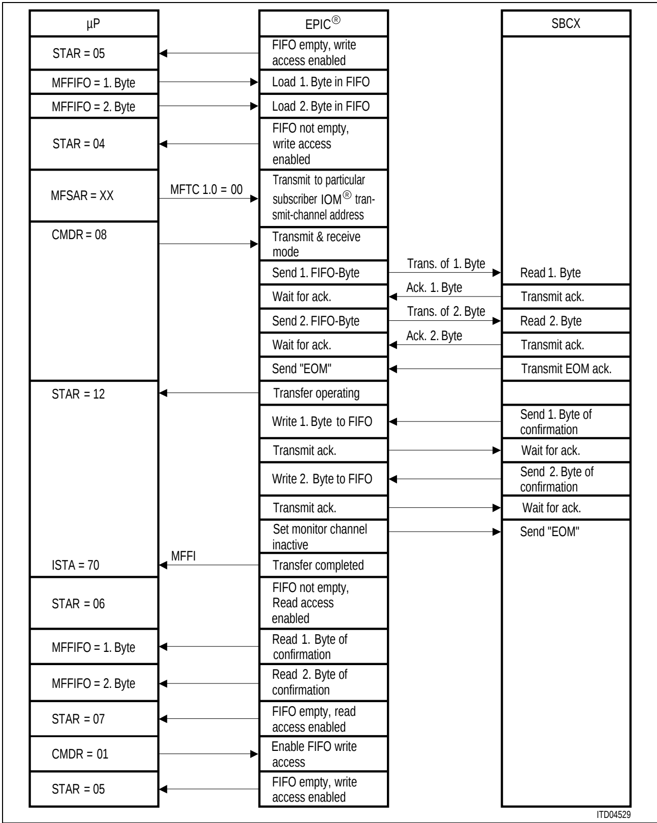
Figure 38 Monitor Channel Handling with EPIC® (all data values hexadecimal)
