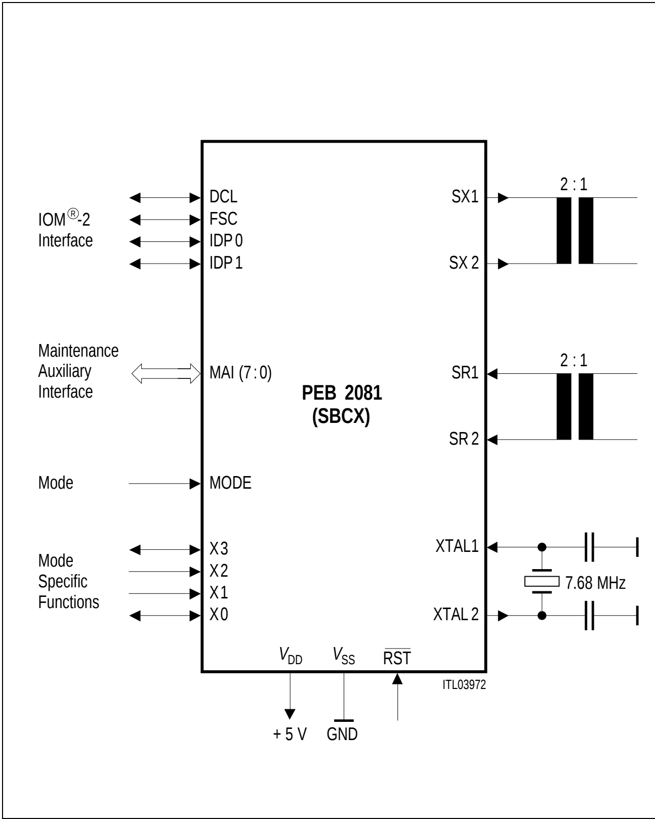
Figure 2 Logic Symbol of the SBCX
