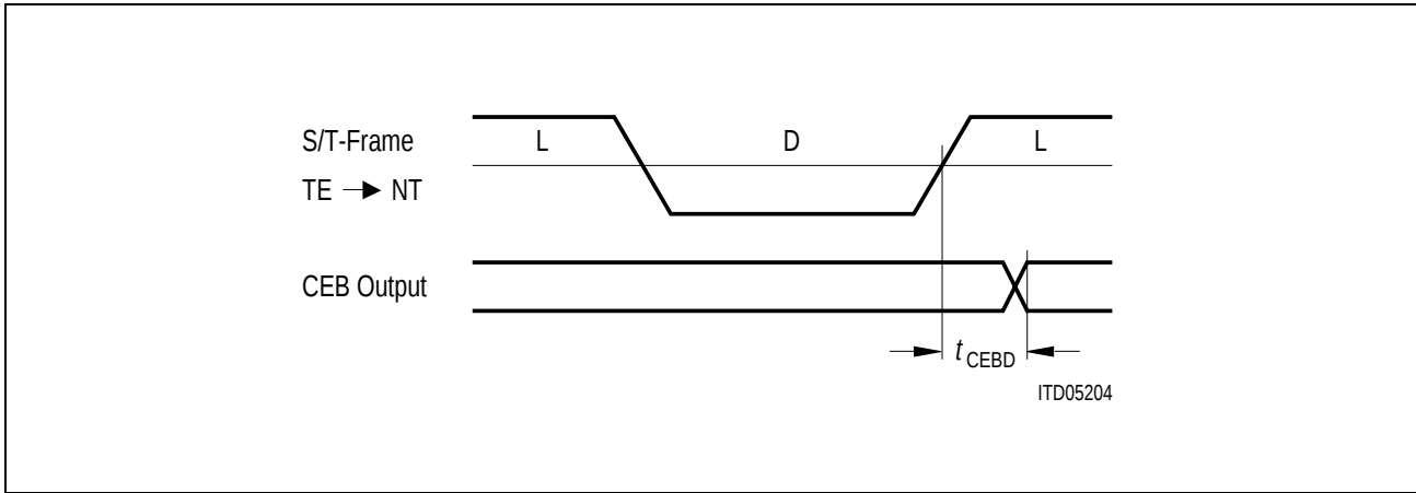
Figure 51 Timing of the CEB Output
