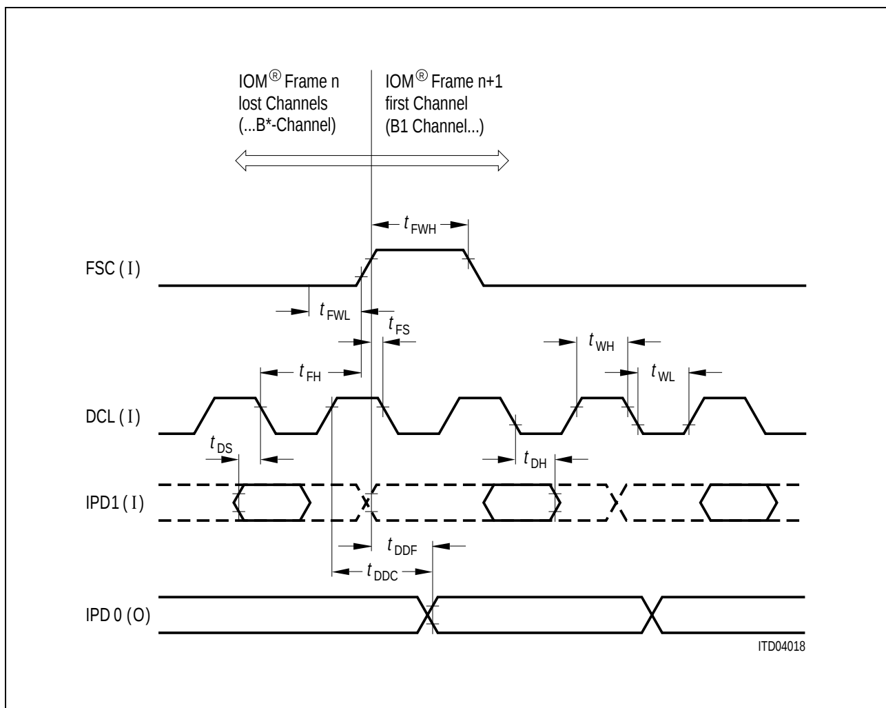
Figure 50 Timing of the IOM ® -2 Interface in NT / LT-S and LT-T Mode
