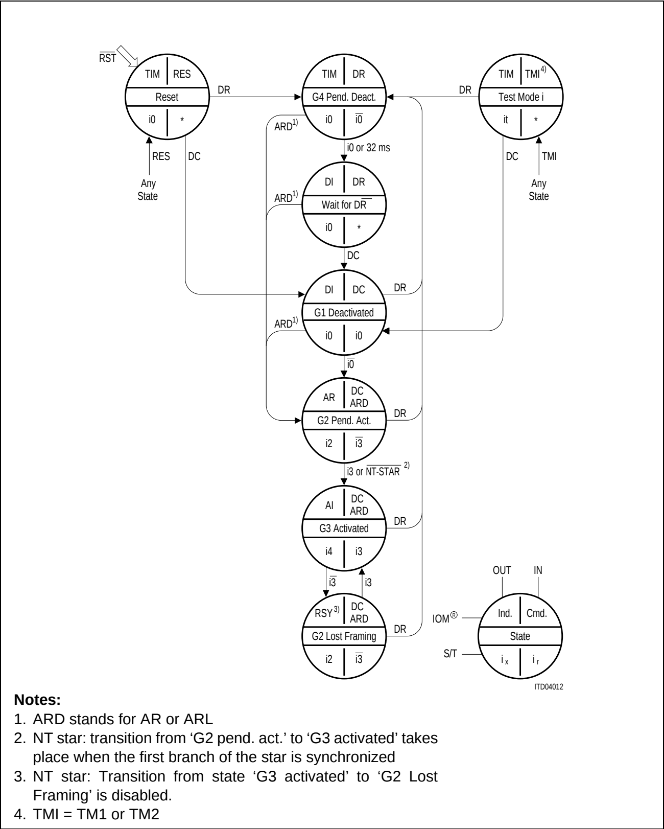
Figure 68 State Transition Diagram in LT-S Mode
