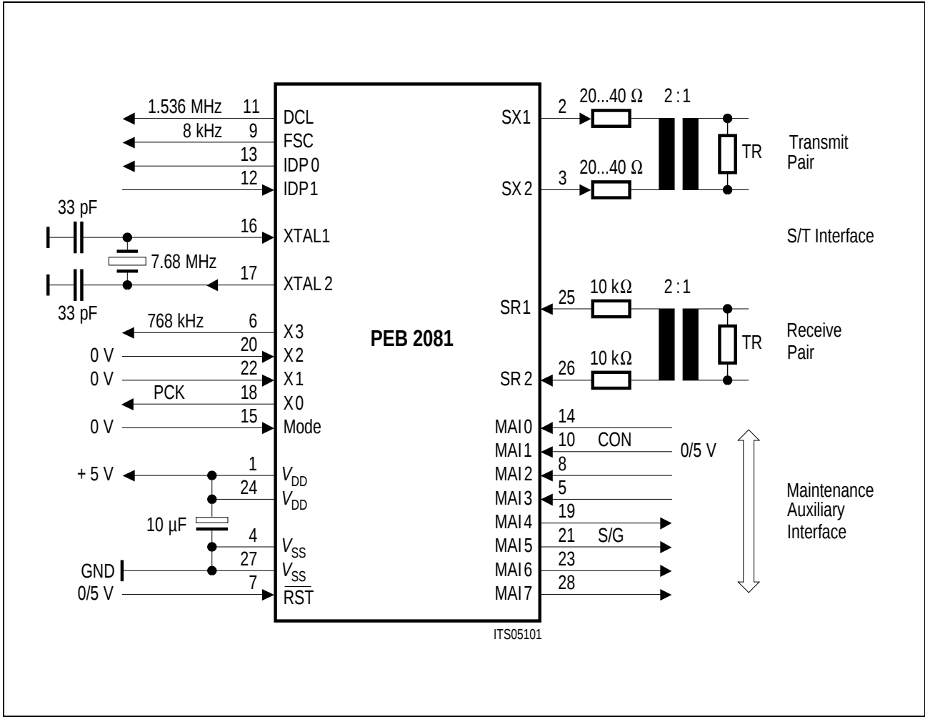
Figure 6 SBCX in TE Mode
