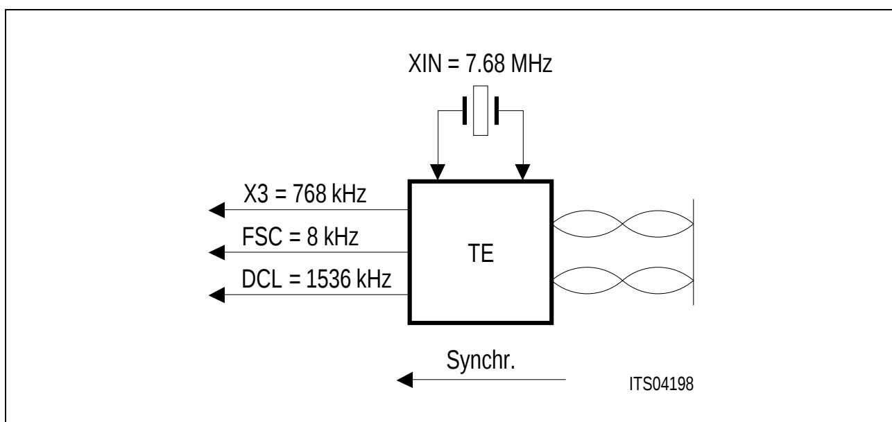
Figure 23 Clock Generation for TE Mode
