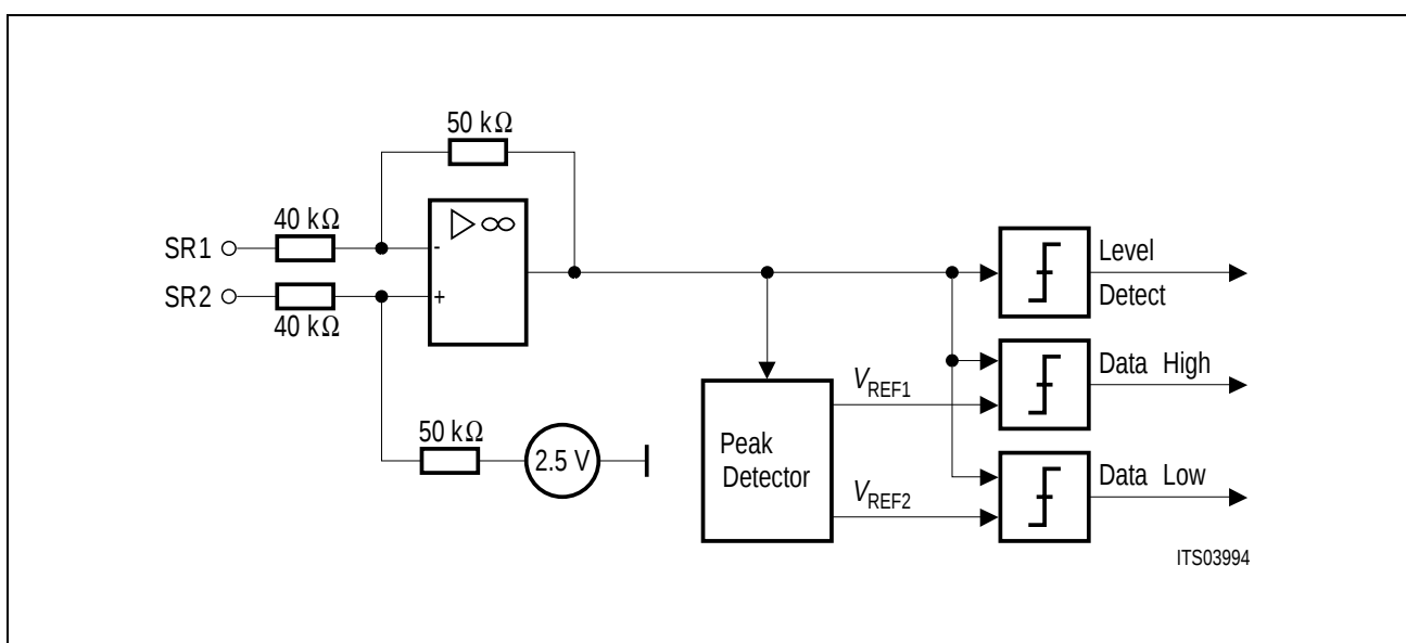
Figure 76 Receiver Circuit
