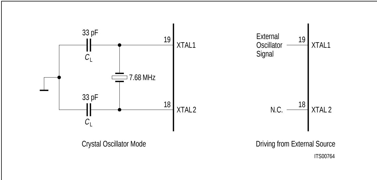
Figure 75 Recommended Oscillator Circuits
