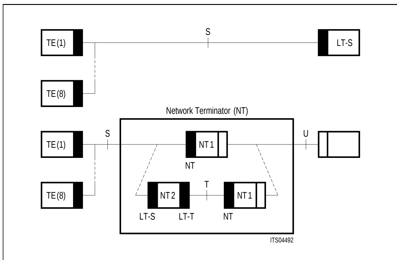
Figure 4 Operating Modes of the SBCX in the ISDN Basic Access Architecture
