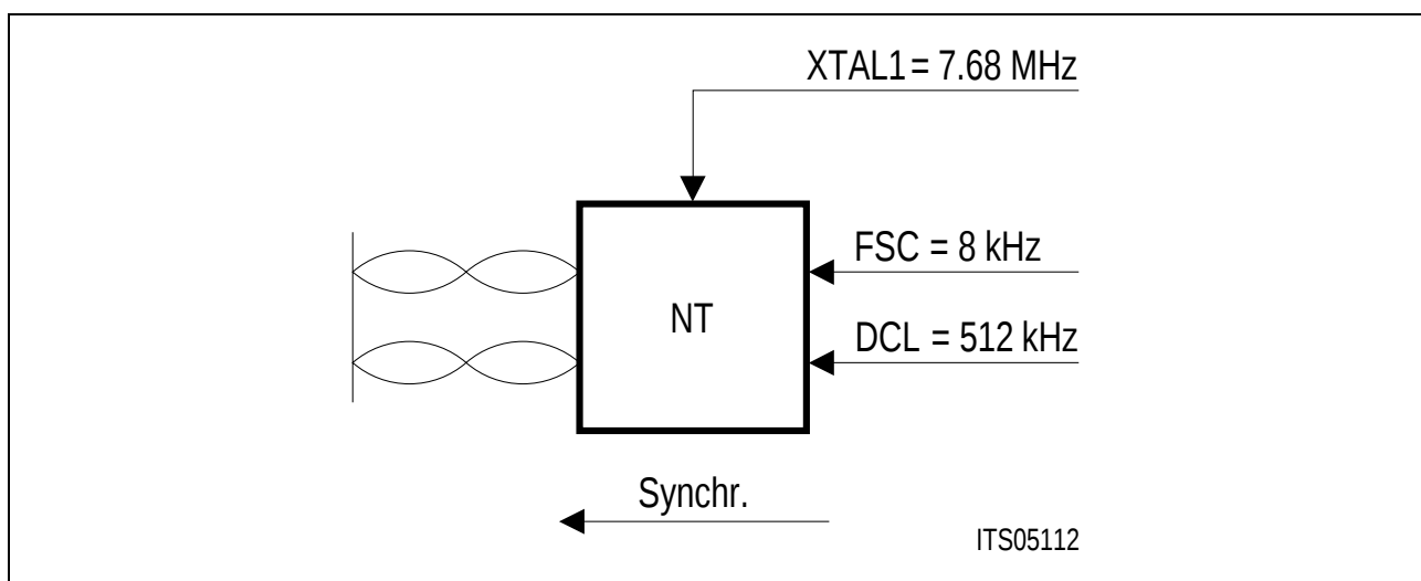
Figure 24 Clocks Generation in NT Mode
