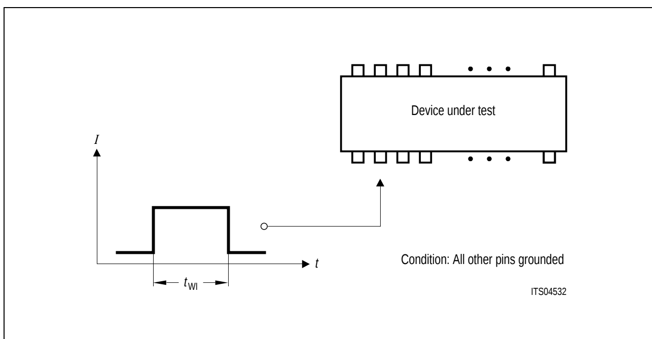
Figure 83 Test Condition for Maximum Input Current
