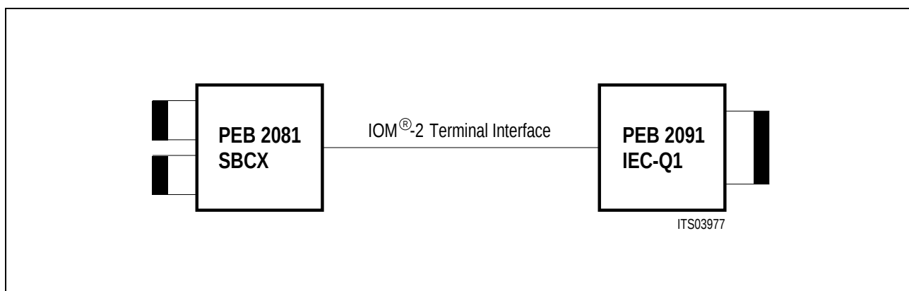
Figure 7 Basic Network Terminator (NT1)
