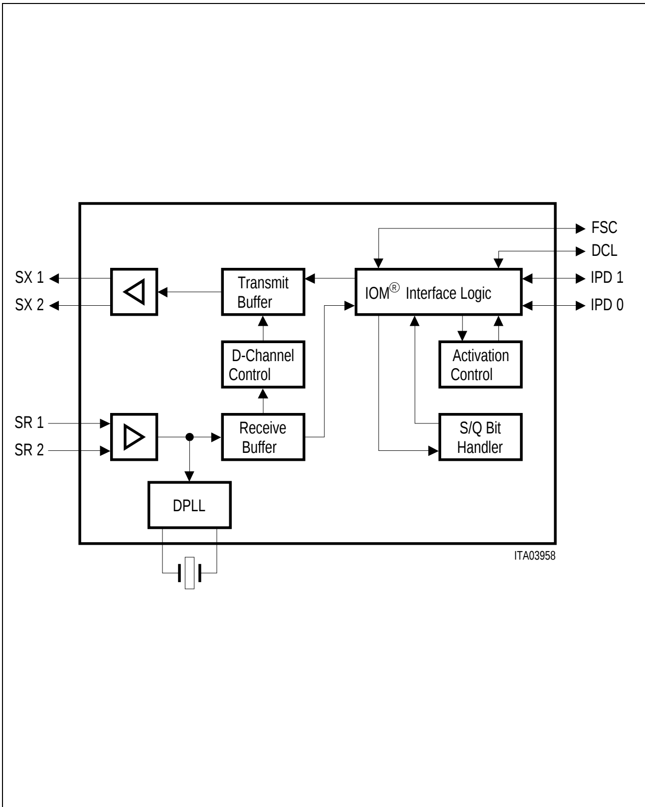
Figure 3 Block Diagram of the SBCX
