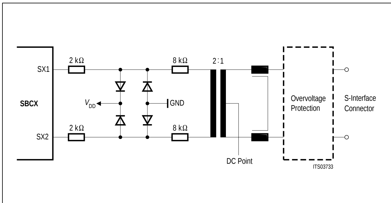
Figure 81 External Circuitry Receiver
