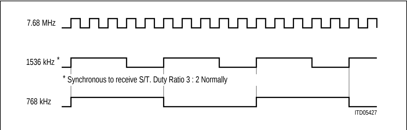
Figure 74 Phase Relationships of TE Clock Signals
