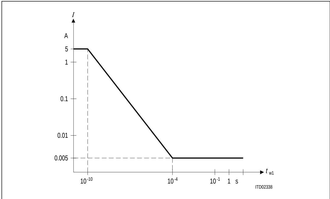
Figure 85 Destruction Limits Receiver Input Current
