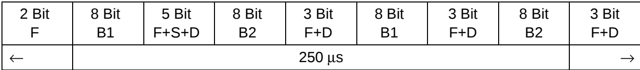
Figure 40 S-Frame Structure
