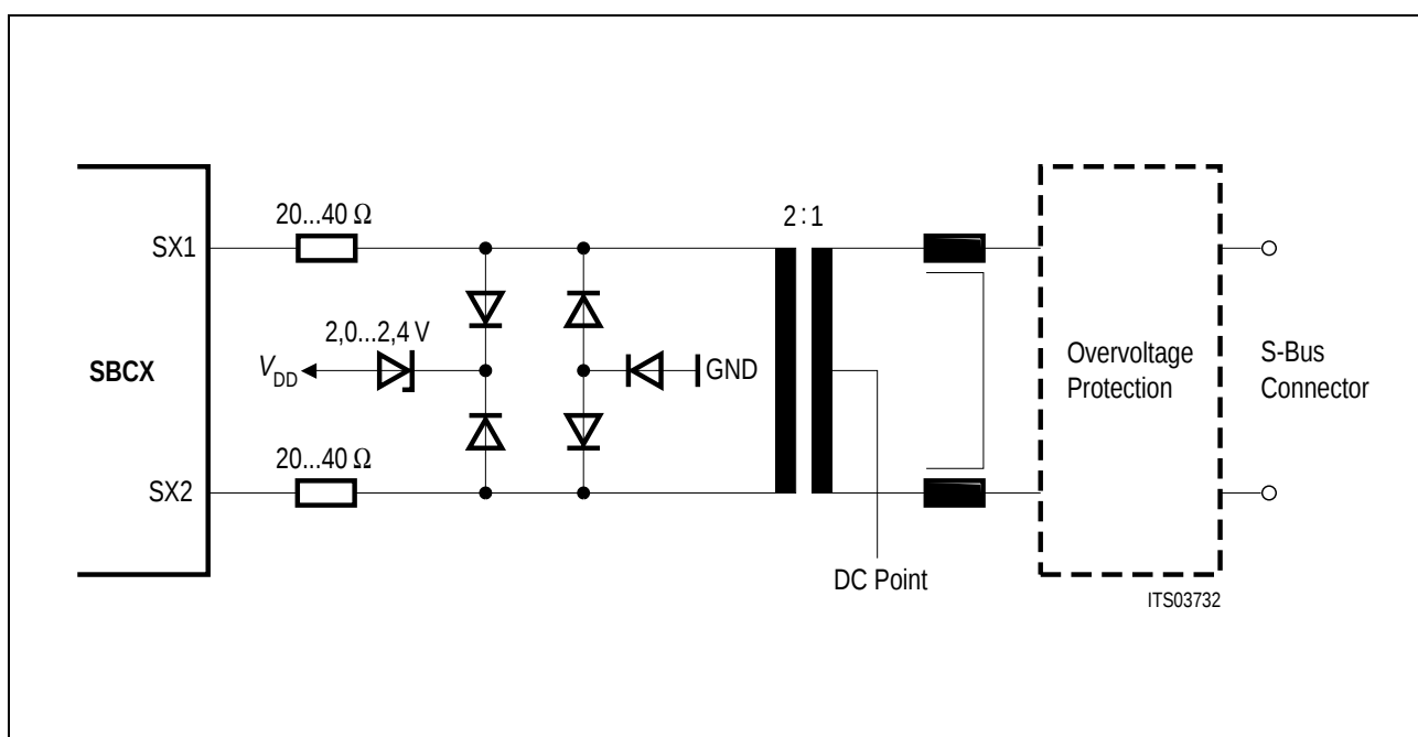
Figure 80 External Circuitry Transmitter
