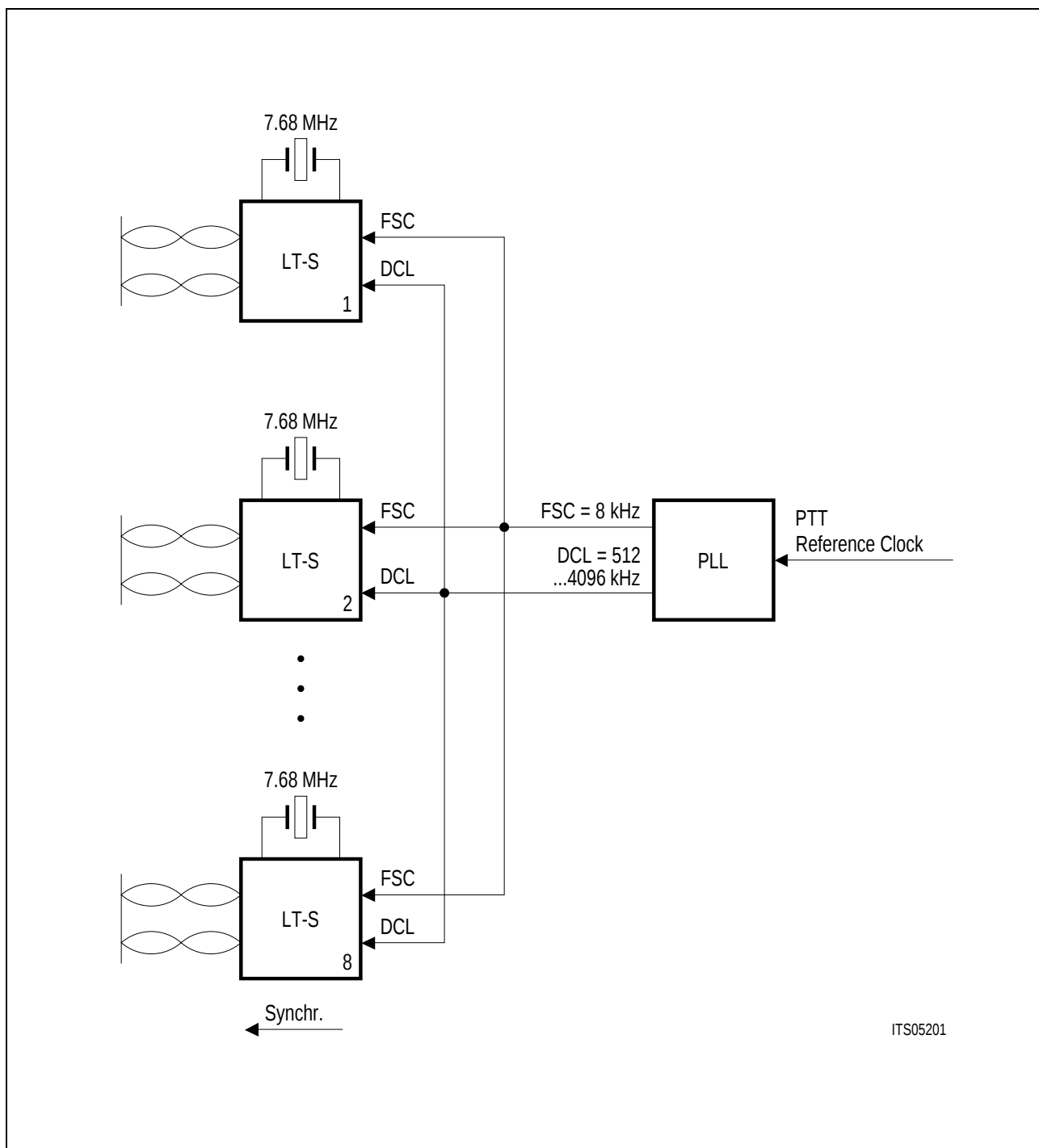
Figure 26 Clock Generation in LT-S Mode
