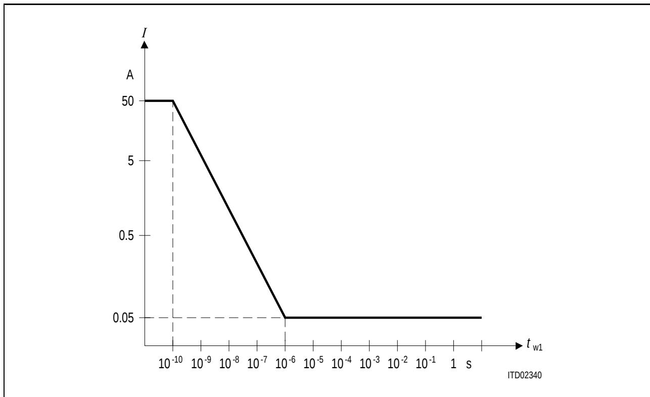
Figure 84 Destruction Limits Transmitter Input Current
