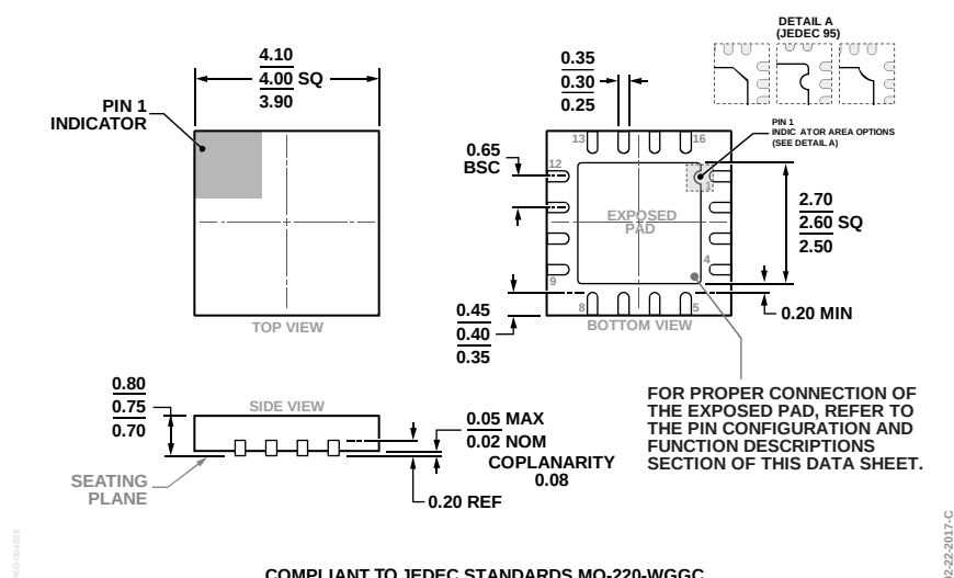
Figure 48. 16-Lead Lead Frame Chip Scale Package [LFCSP] 4 mm × 4 mm Body and 0.75 mm Package Height (CP-16-17)
