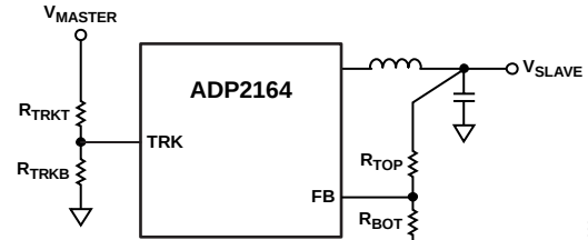
Figure 39. Voltage Tracking
