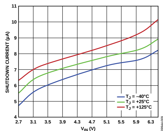
Figure 9. Shutdown Current vs. V_{IN}
