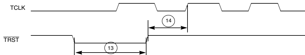
Figure 14. TRST Timing
