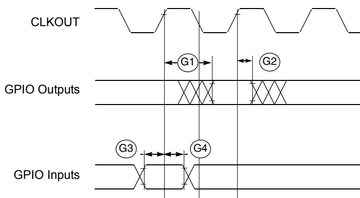
Figure 6. GPIO Timing
