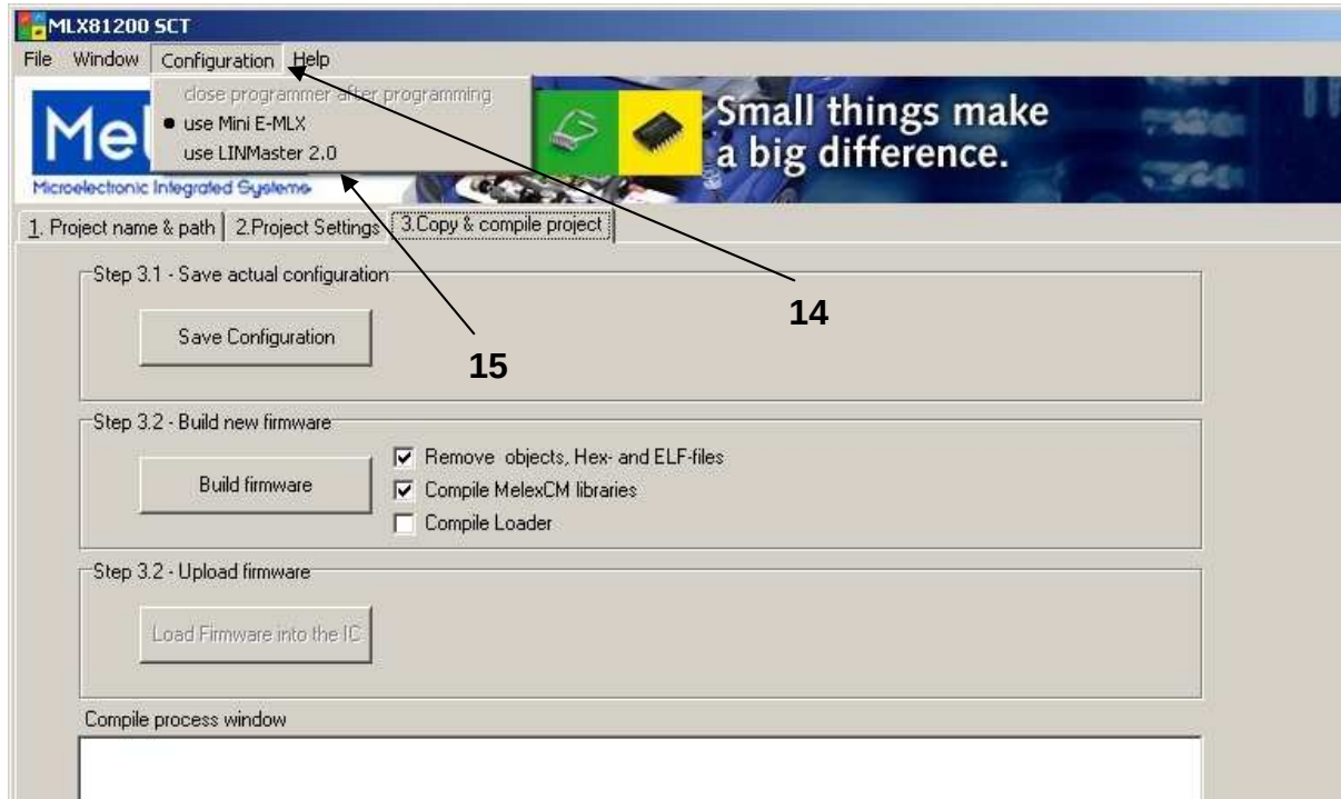
Fig. 21 MLX81200 SCT – configure the hardware in use
