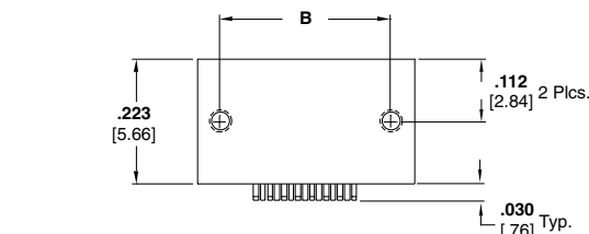
Receptacle Assembly Drawing Number 1589484
