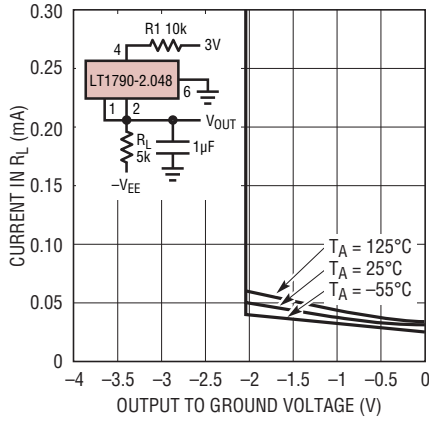
–2.048V Characteristics
