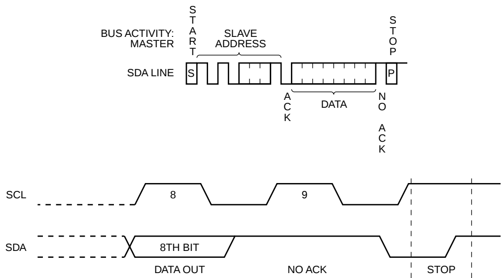
Figure 8. Immediate Address Read Timing
