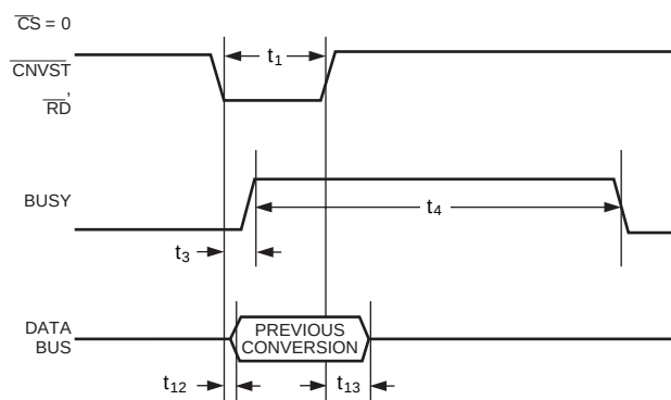
Figure 15. Slave Parallel Data Timing for Reading
