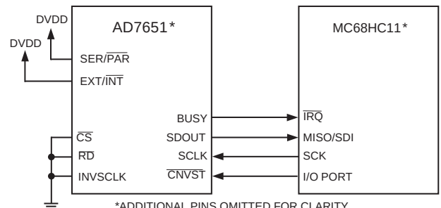
Figure 21. Interfacing the AD7651 to SPI Interface
