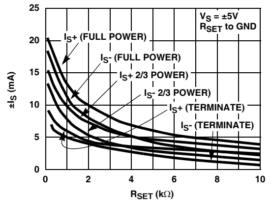
FIGURE 34. I_S vs R_{SET}
