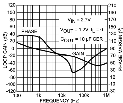
FIGURE 3. Gain-Bandwidth Plot for No Load
