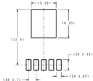
TO-263 THIN 5-Lead, Molded, Surface Mount Package NS Package Number TJ5A
