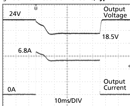
Fig. 26-3 Peak load 6.8A for 50ms, typ.
