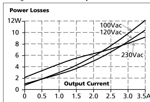
Fig. 10-4 Losses vs. input voltage, 24V, 3.4A
