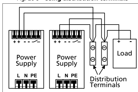
Fig. 26-9 Using distribution terminals
