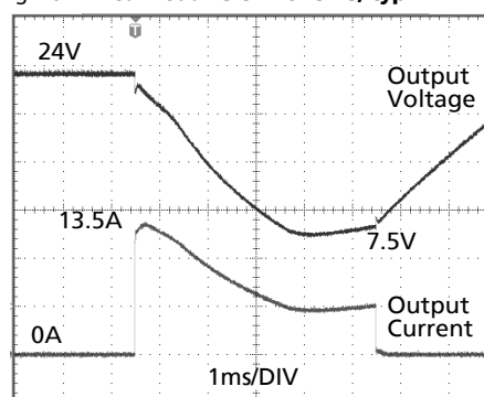
Fig. 26-4 Peak load 13.5A for 5ms, typ.
