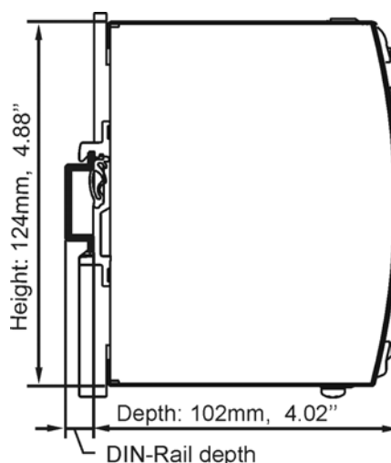
Fig. 23-2 Side view
