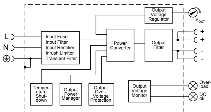
Fig. 11-1 Functional diagram
