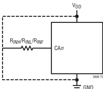
Test Circuit 2
