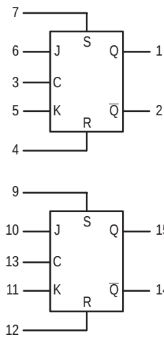
BLOCK DIAGRAM
