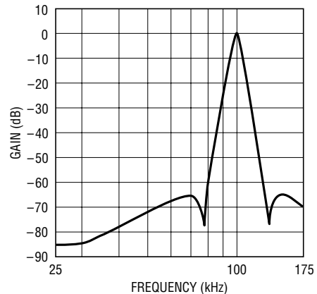
Amplitude Response
