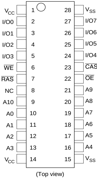
HM5117805BTT/BLTT Series HM5117805BTS/BLTS Series
