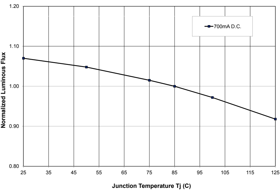
Figure 4. Relative light output vs. junction temperature.
