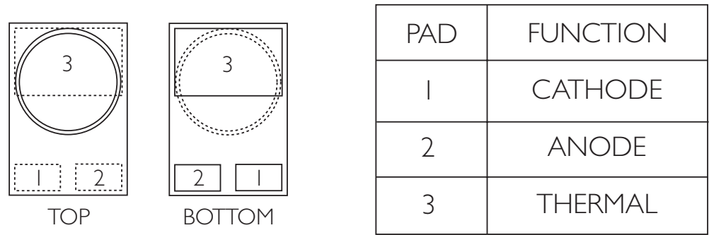
Figure 2. Pad configuration.
