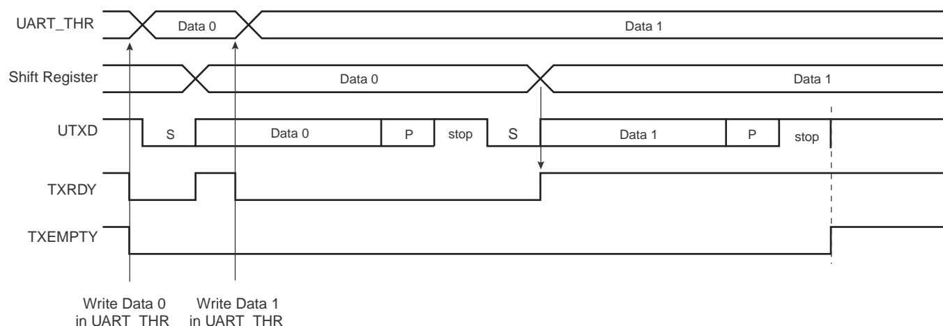
Figure 33-10. Transmitter Control
