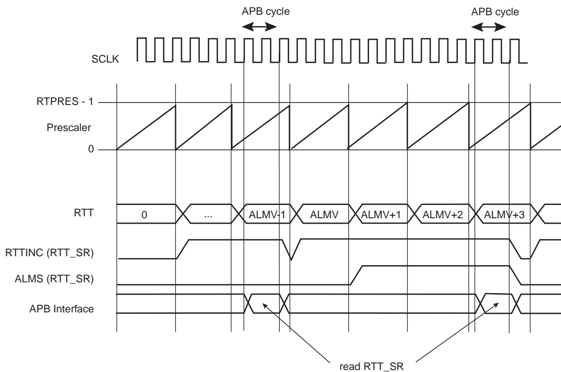
Figure 16-2. RTT Counting
