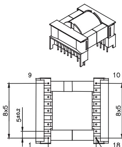
Bottom View (Pin side)
