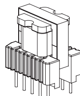
E 19 reinforced insulation creepage distances: 6mm
