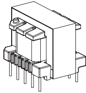
EI 28 reinforced insulation creepage distances: 6mm
