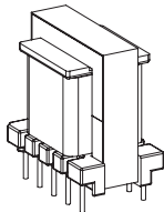
EF 25 reinforced insulation creepage distances: 6mm
