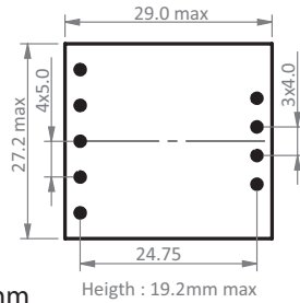
E 25 reinforced insulation creepage distances: 8mm
