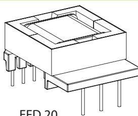
EFD 20 reinforced insulation creepage distances: 6mm
