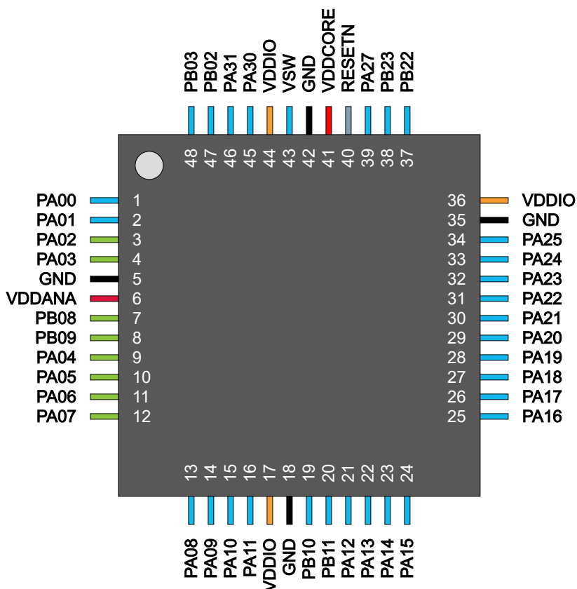
Figure 4-1. 48-Pin QFN (1) Package
