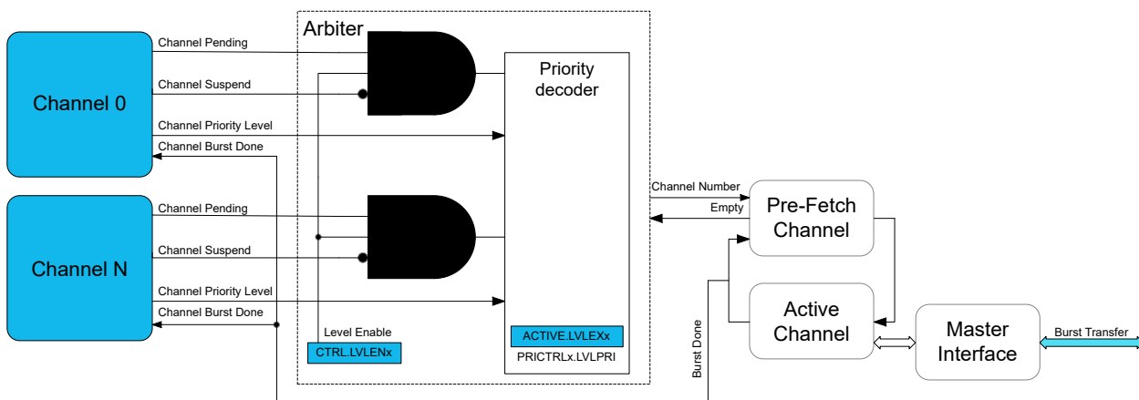
Figure 22-4. Arbiter Overview
