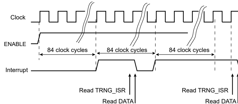
Figure 44-2. TRNG Data Generation Sequence
