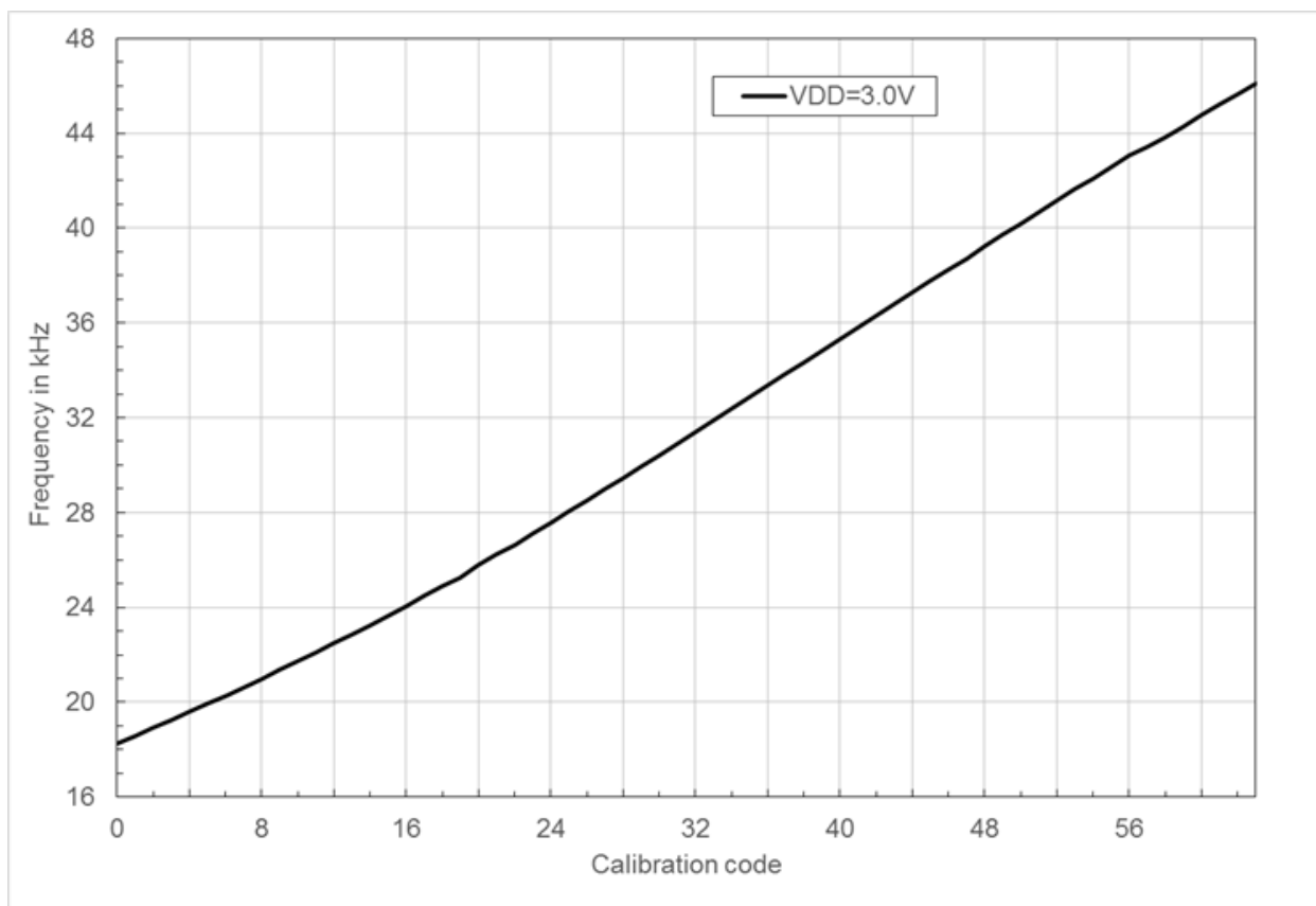
Figure 54-8. Average Frequency Versus Calibration Code Value, VDD = 3V
