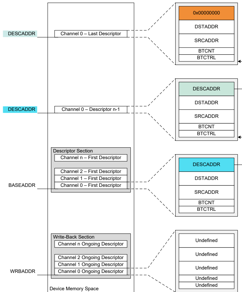
Figure 22-3. Memory Sections
