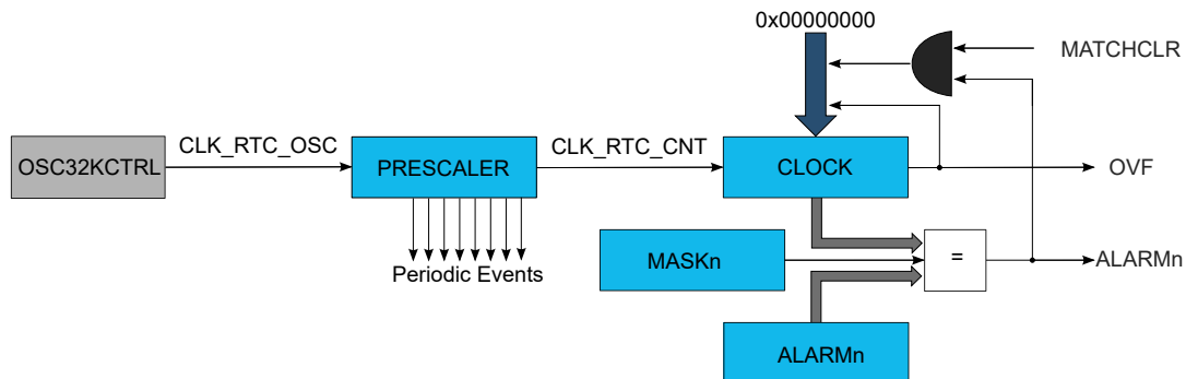
Figure 21-3. RTC Block Diagram (Mode 2 — Clock/Calendar)
