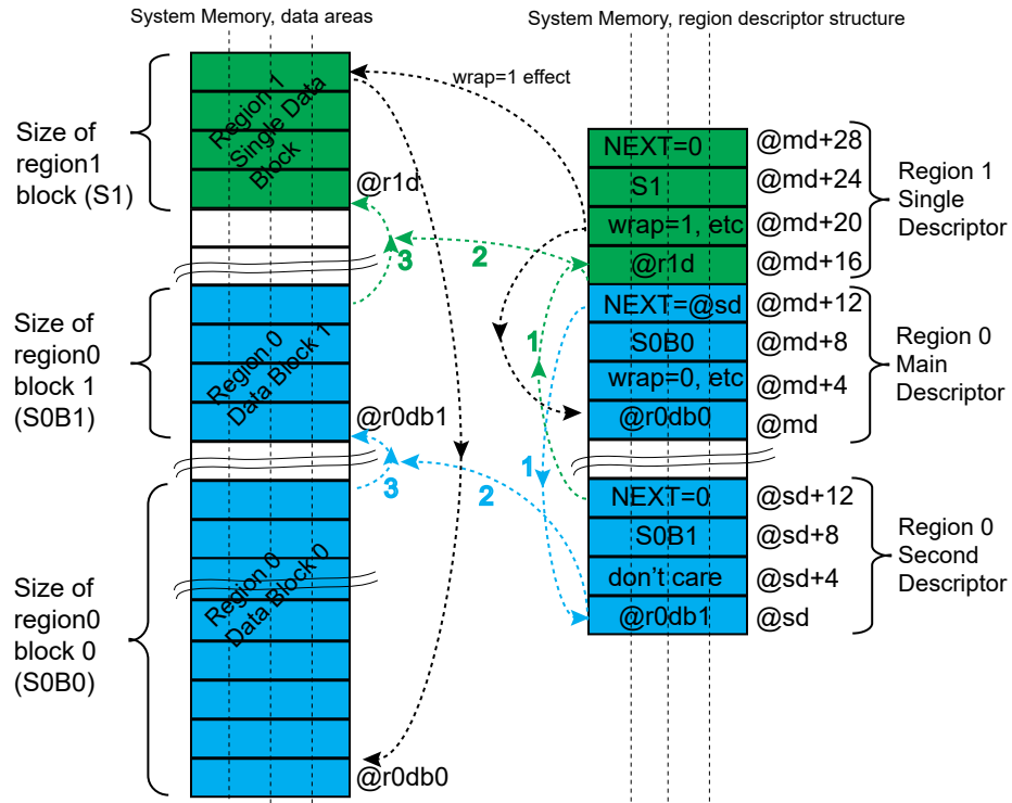
Figure 26-4. Example - Monitoring of 3 Memory Data Blocks (Defined as 2 Regions)
