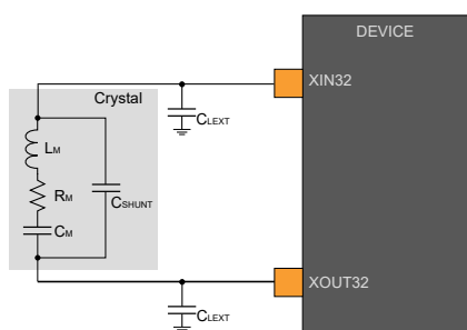
Figure 54-7. Oscillator Crystal Connection
