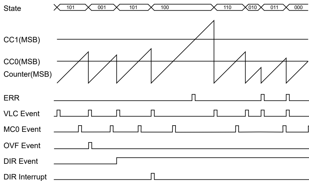
Figure 53-9. Hall Waveforms
