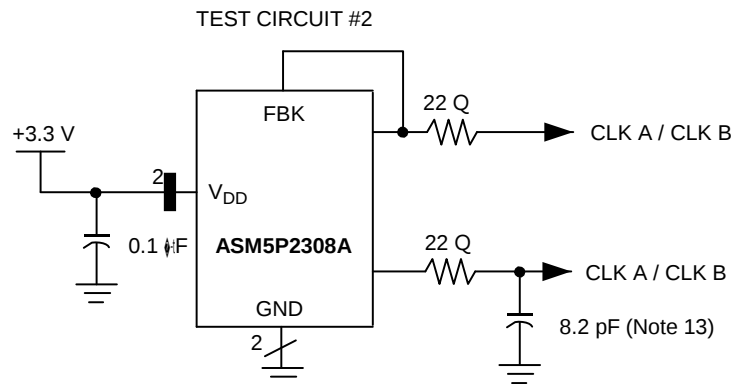
Figure 8. Test Circuits
