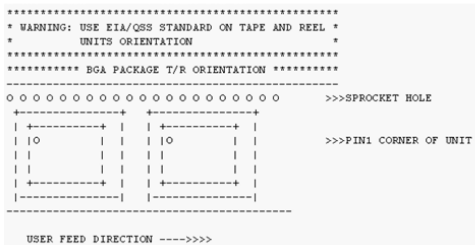
Figure A-6. Tape and Reel BGA Pin 1 Location
