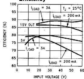
Efficiency
