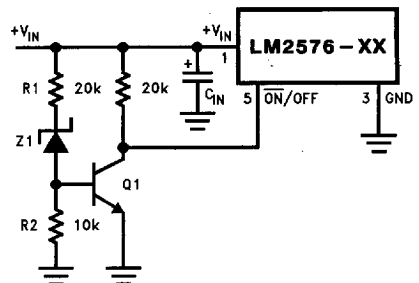
FIGURE 12. Undervoltage Lockout for Buck Circuit
