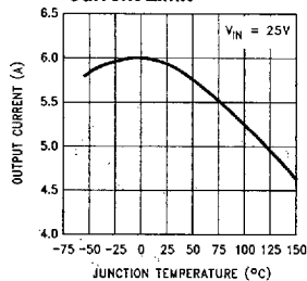
Current Limit
