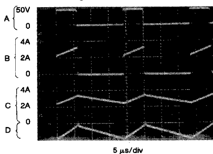
Switching Waveforms
