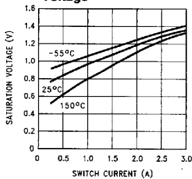
Switch Saturation Voltage
