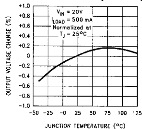
Normalized Output Voltage
