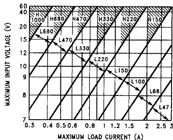
FIGURE 4. LM2576(HV)-5.0
