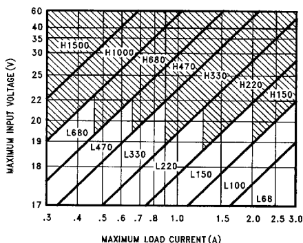
FIGURE 6. LM2576(HV)-15
