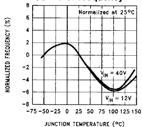
Oscillator Frequency
