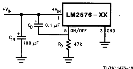
FIGURE 14. Delayed Startup
