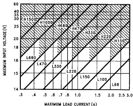
FIGURE 5. LM2576(HV)-12
