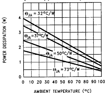
Maximum Power Dissipation (TO-263) (See Note 10)
