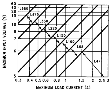
FIGURE 3. LM2576(HV)-3.3
