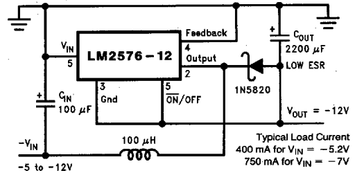
FIGURE 11. Negative Boost
