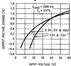
Line Regulation
