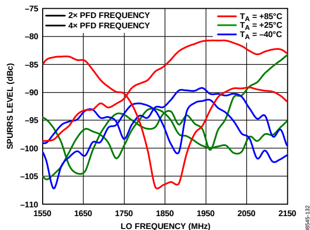
Figure 33. PLL Reference Spurs vs. LO Frequency (2x PFD and 4x PFD)
