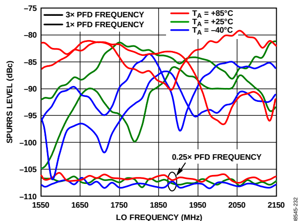
Figure 34. PLL Reference Spurs vs. LO Frequency (0.25x PFD, 1x PFD, and 3x PFD)
