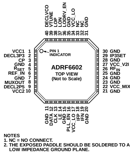
Figure 3. Pin Configuration
