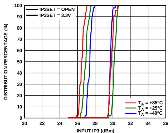
Figure 29. Input IP3
