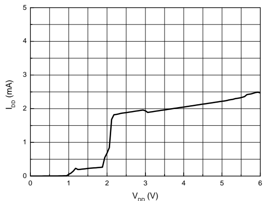
Supply Current I_{DD} vs. Supply Voltage V_{DD}
