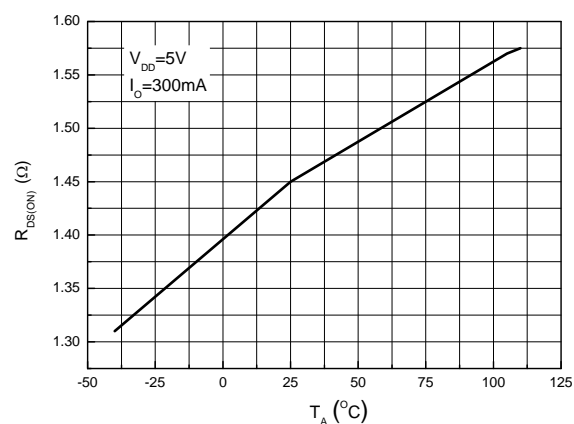
High+Low Side R_{DS(ON)} vs. Operating Temperature T_A
