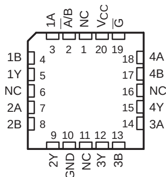
SN54HC157 . . . FK PACKAGE (TOP VIEW)
