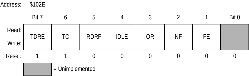
Figure 7-6. Serial Communications Status Register (SCSR)
