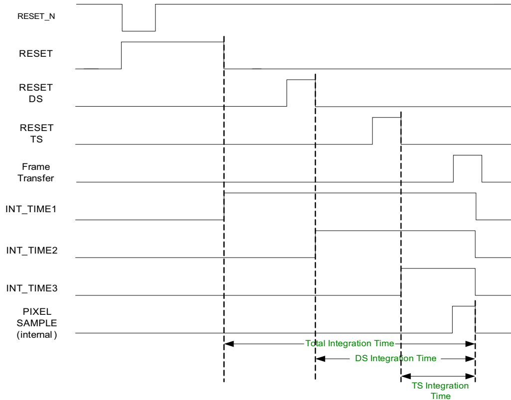
Figure 15. INT_TIME Timing
