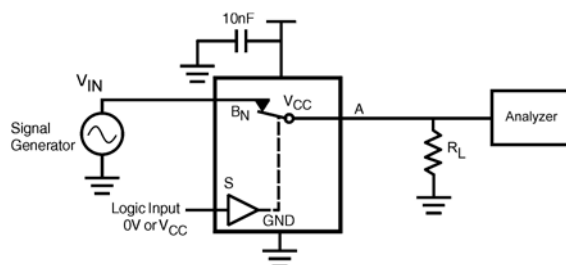
FIGURE 10. Harmonic Distortion
