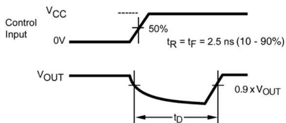
FIGURE 5. Break-Before-Make Timing
