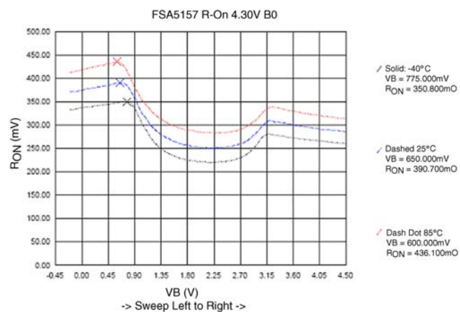
FIGURE 3. R ON Switch On Resistance, I ON = 100mA, V CC = 4.3V
