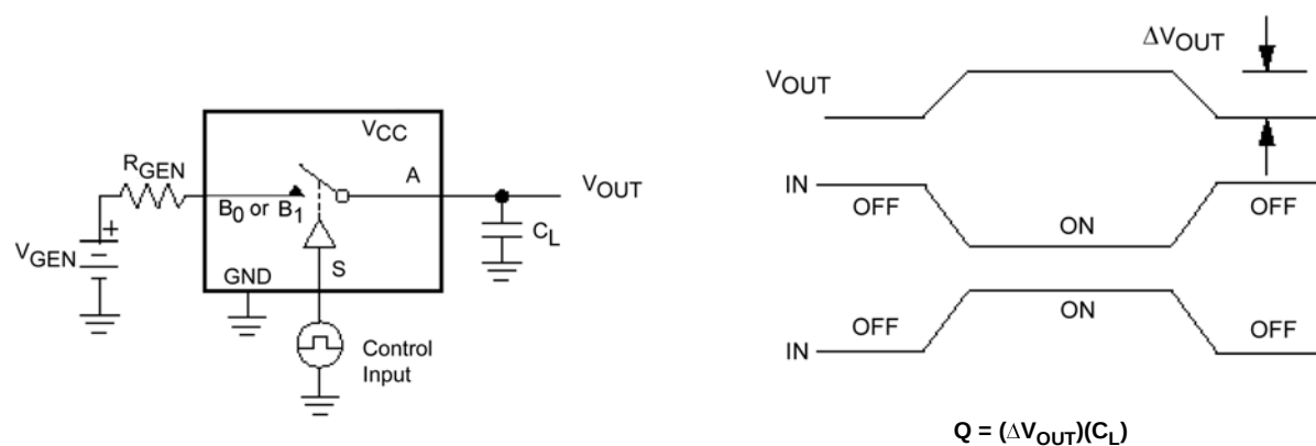
FIGURE 7. Charge Injection
