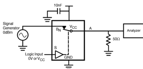
FIGURE 9. Bandwidth
