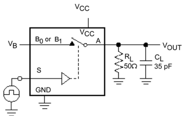
FIGURE 4. Turn-On/Turn-Off Timing
