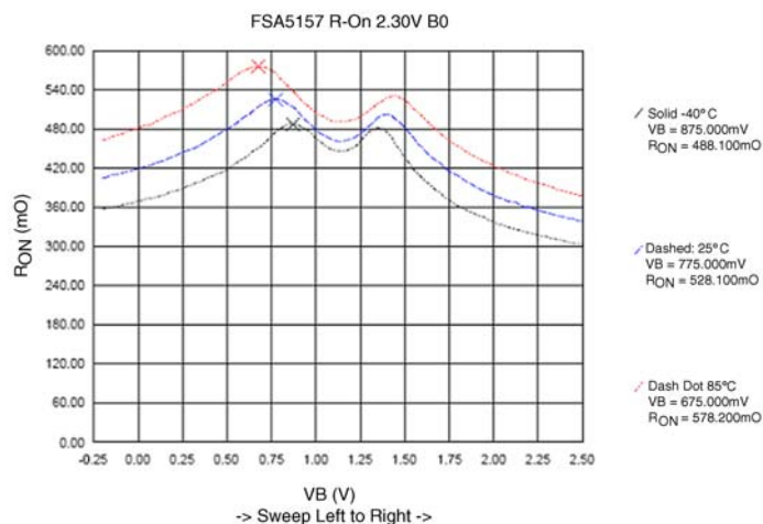
FIGURE 1. R ON Switch On Resistance, I ON = 100mA, V CC = 2.3V
