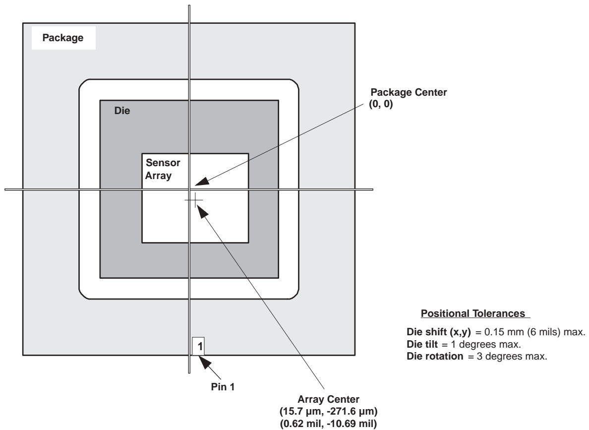
Figure 22 OV9625/OV9121 Sensor Array Center
