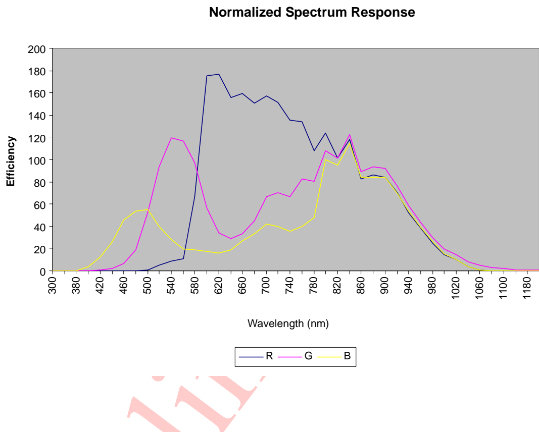
Figure 20 OV9625/OV9121 Light Response
