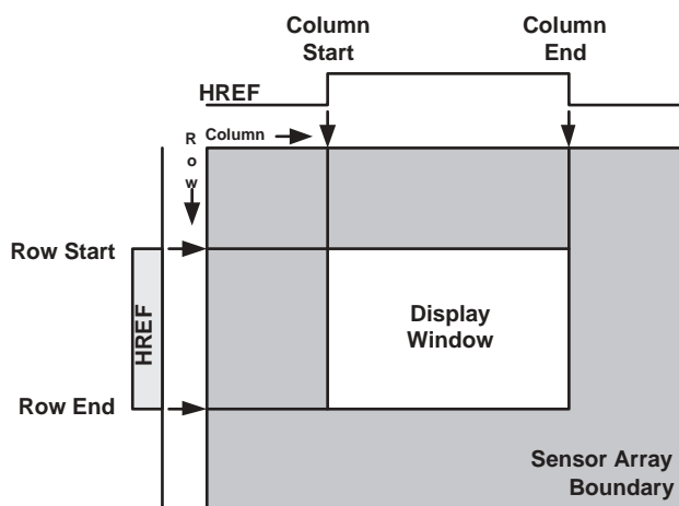
Figure 4 Windowing
