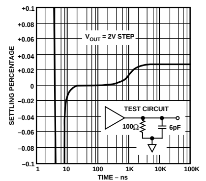
Figure 11. Long-Term Settling Time
