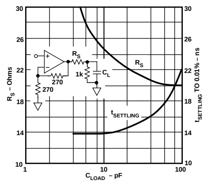
Figure 14. Settling Time vs. Capacitive Load
