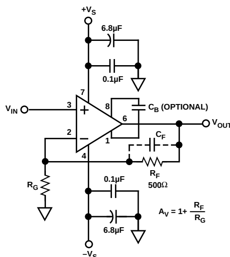
Figure 2. Noninverting Gain Connection Diagram
