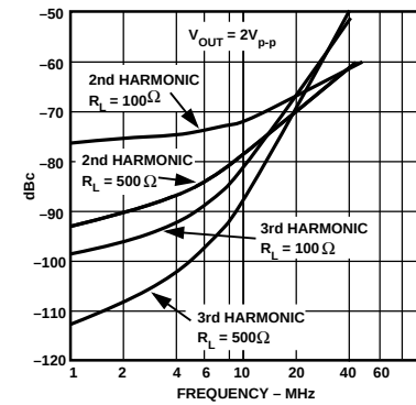
Figure 6. Harmonic Distortion vs. Frequency
