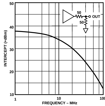
Figure 7. Third Order Intercept
