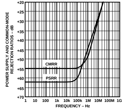
Figure 8. CMRR and PSRR vs. Frequency
