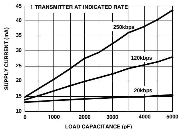
FIGURE 21. ISL4244E SUPPLY CURRENT vs LOAD CAPACITANCE WHEN TRANSMITTING DATA
