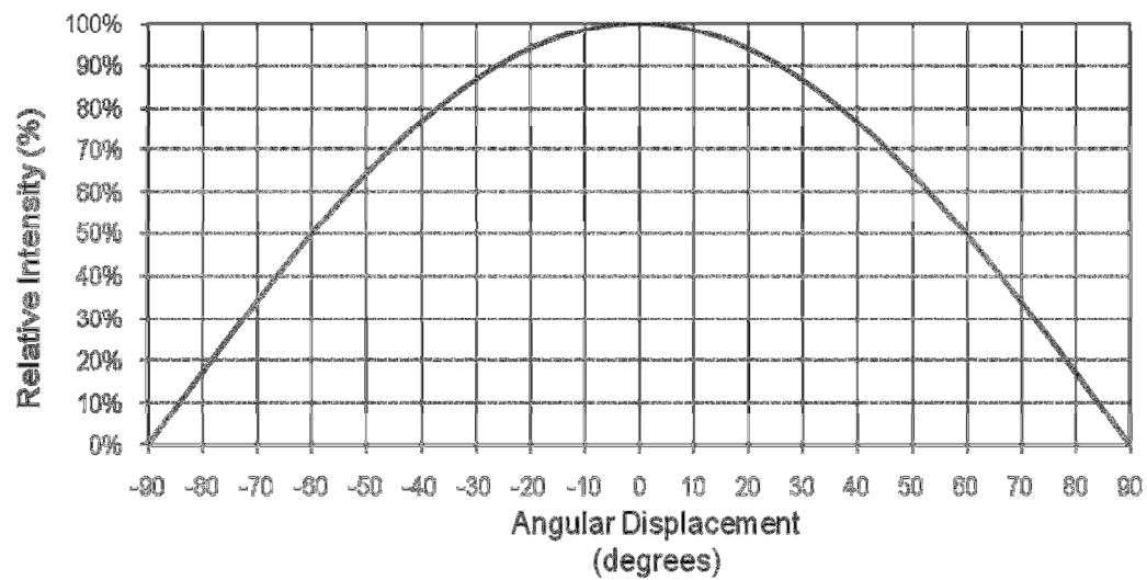
Figure 2: Typical Spatial Radiation Pattern
