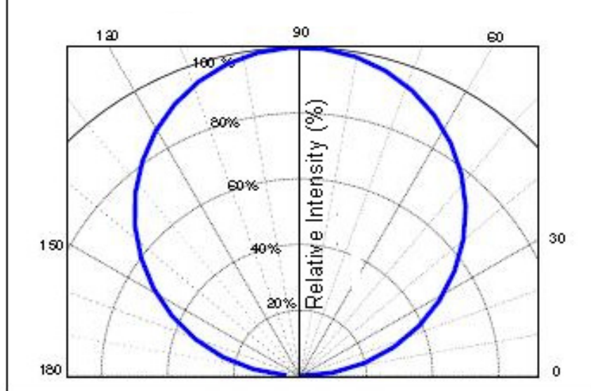
Figure 3: Typical Polar Radiation Pattern
