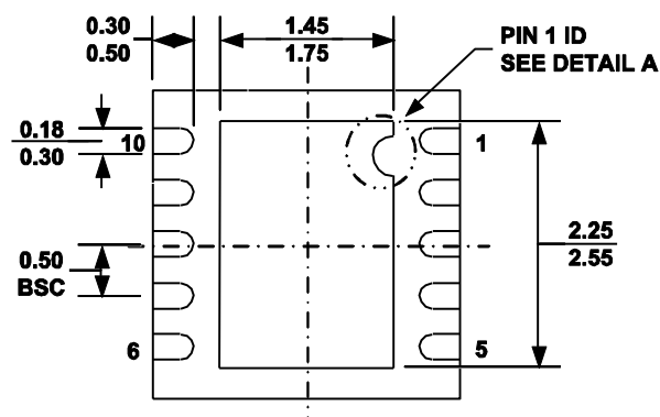
QFN-10 (3mmx3mm)
