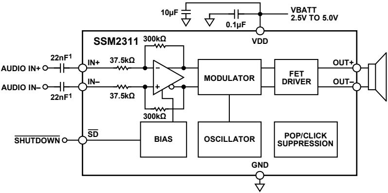
Figure 43. Differential Input Configuration
