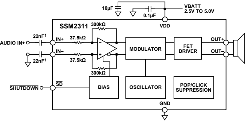
Figure 44. Single-Ended Input Configuration
