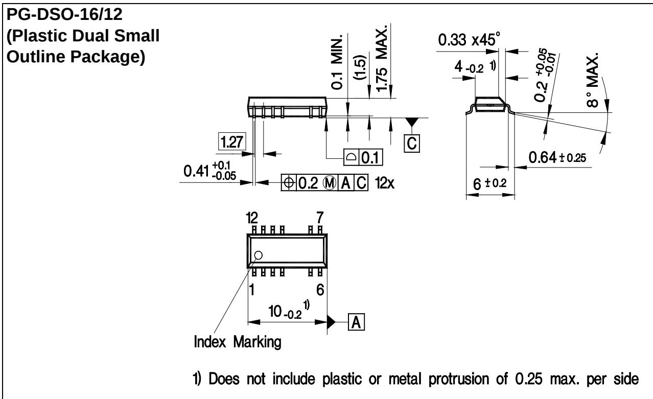
Figure 62 PG-DSO-16/12 (Plastic Dual Small Outline Package)
