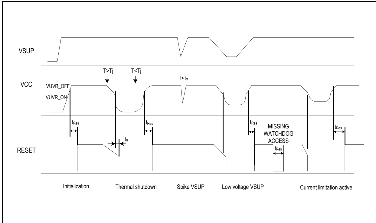
Figure 4. Reset Functionality
