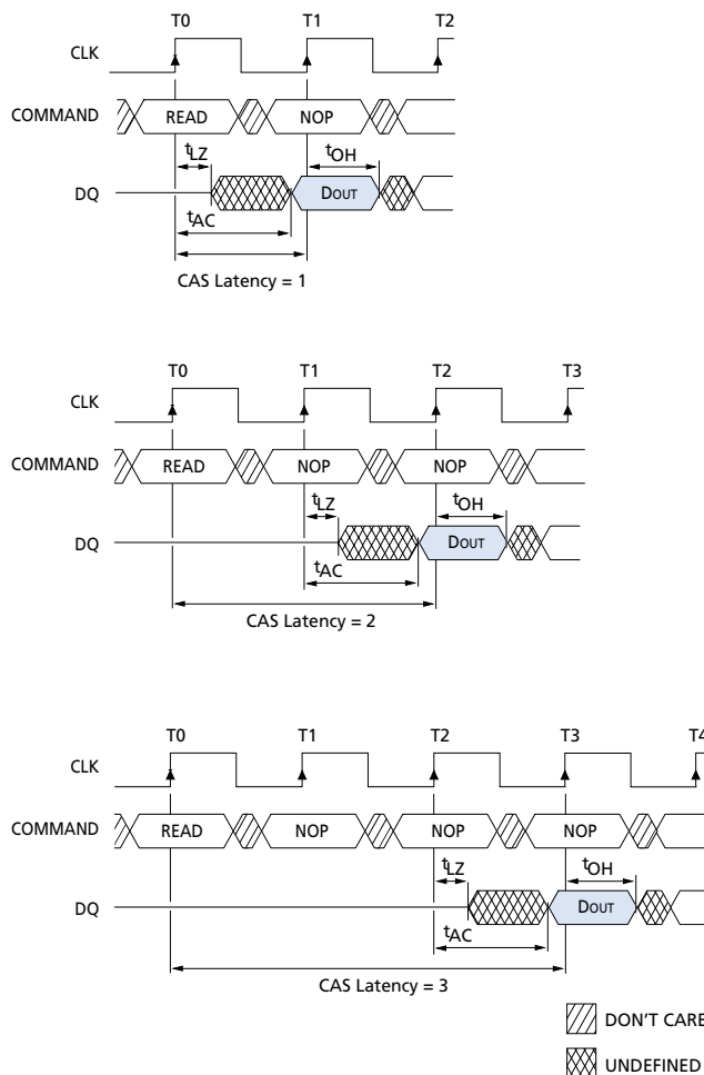
Figure 6 CAS Latency
