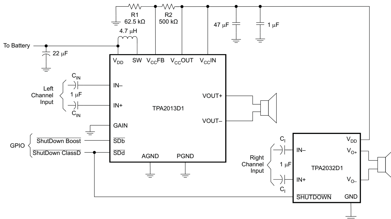
Figure 32. TPA2013D1 in Stereo With the TPA2032D1
