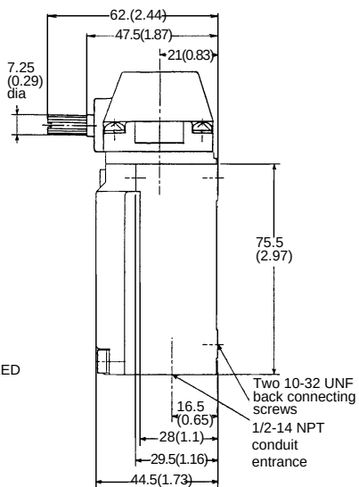
Mounting holes
