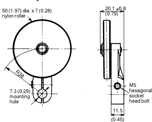
WL-1A106 Nylon Back Mount Roller
